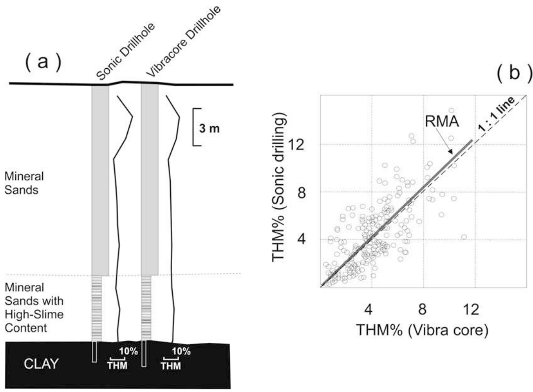
Fig. 11.6 Validation of historic exploration data by twinned holes, Ti-sands project, Madagascar ( THM total heavy minerals) (Reprinted from (Abzalov 2009) with permission of the Canadian Institute of Mining, Metal-
